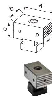
Seri mengene dayama Serial vice resting
